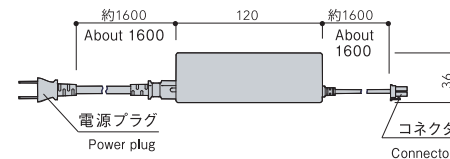
CNSA-120×60×36-2427
