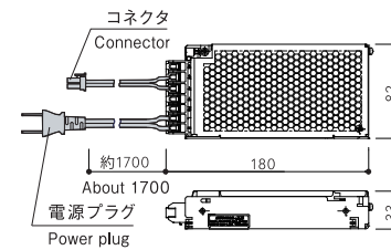
CNSA-180×82×42-2465
